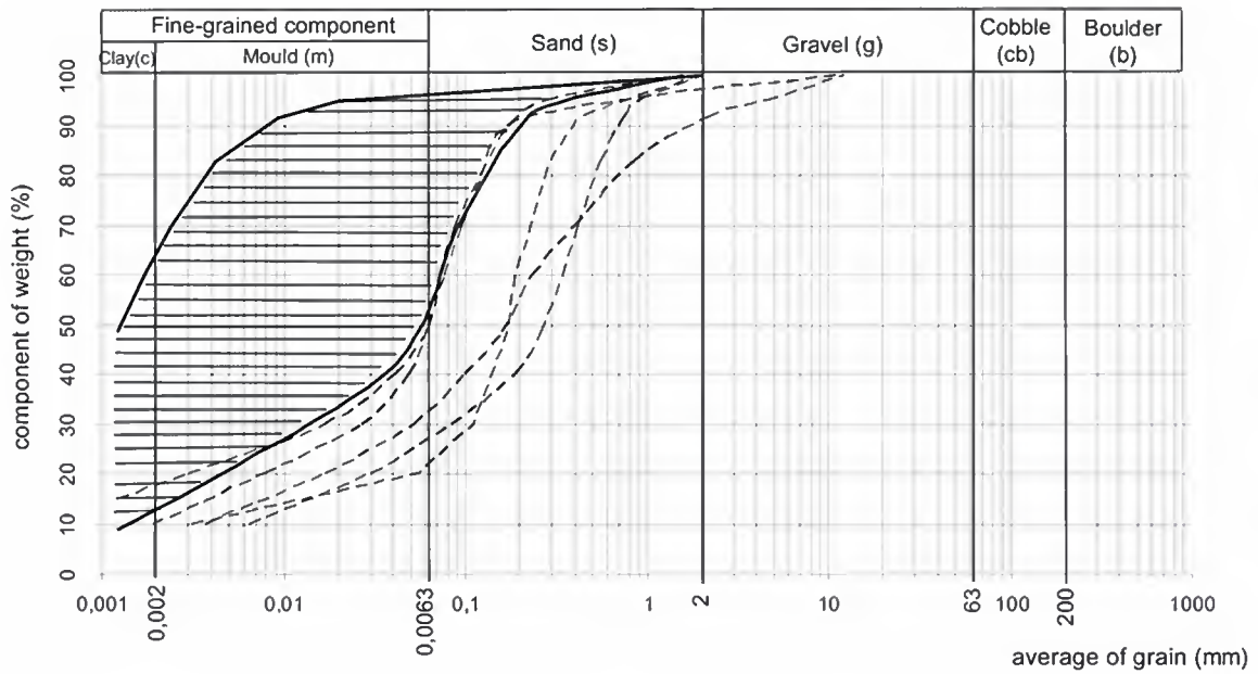
Figure 1. Envelope curves grain-size curves determined soil
